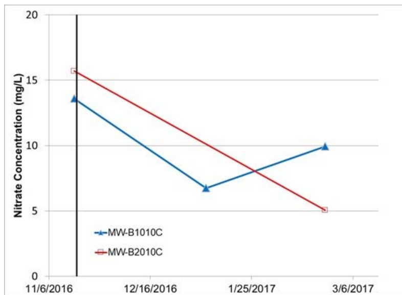
FIGURE 8. Nitrate concentration in two wells approximately 3 meters downgradient of PRB.
