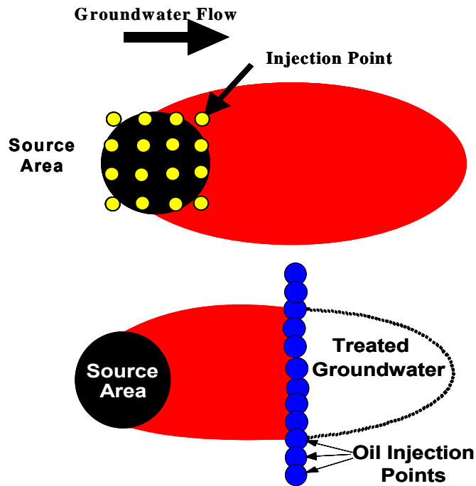
Figure 4.1 Injection Configurations for Using Edible Oil to Treat Contaminated Groundwater in: (a) Source Areas and (b) Biobarriers
