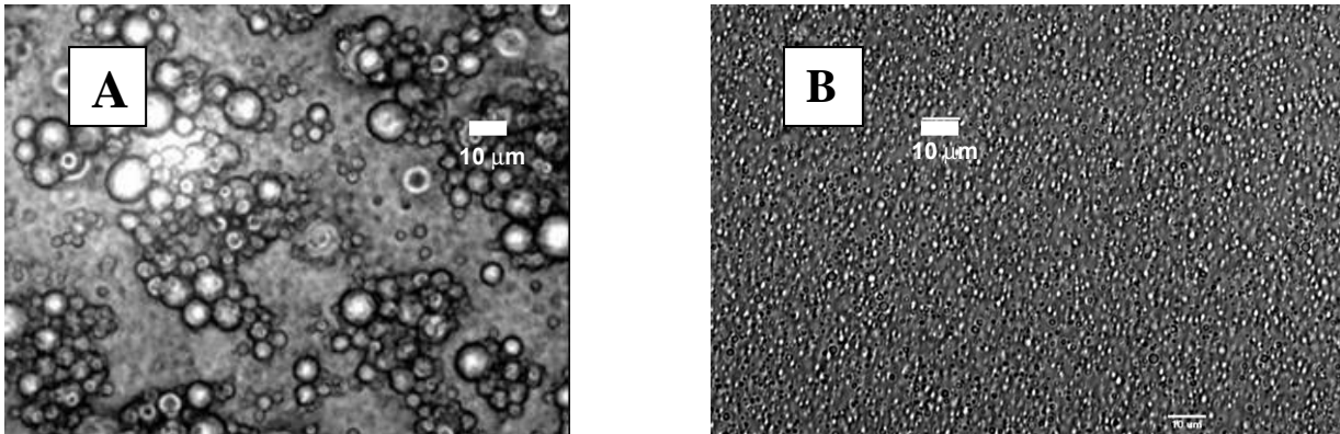
Figure 1.6 Photomicrographs of Oil-in-Water Emulsions: (a) produced in the field with a high shear mixer and (b) a pre-mixed emulsion (white scale bar is 10 microns)
